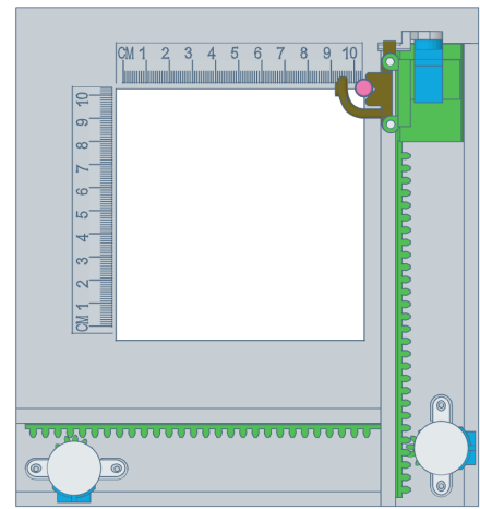
1.2 - Vista Superior
