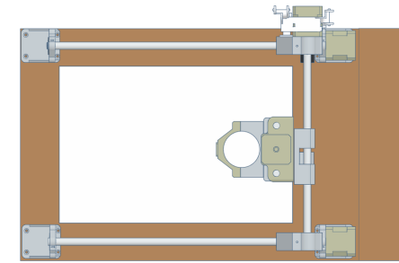
1.2 - Vista Superior
