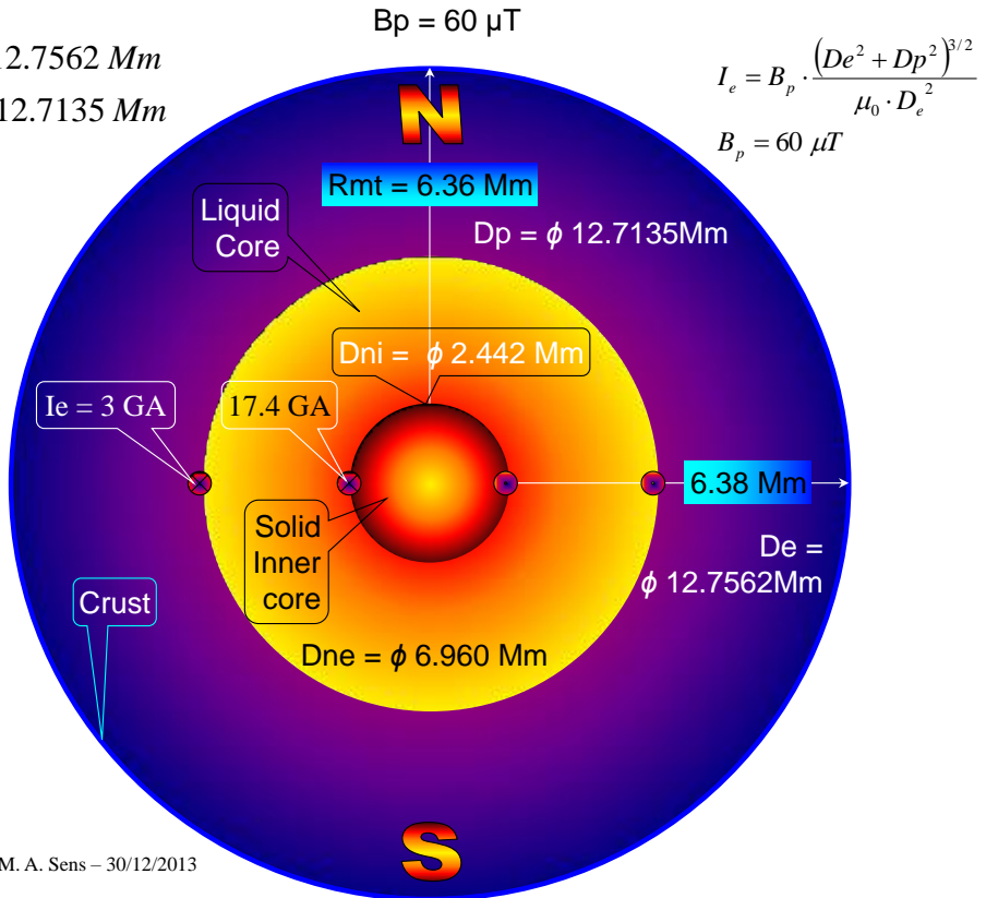
Figure 1 - Geomagnetism Generated By Electric Current in the Core
