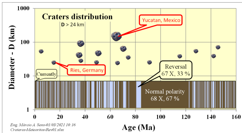
Figure 2 - Correlation of Geomagnetic Reversals with Asteroid Impacts
