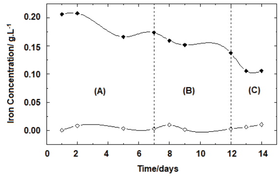
Figure 7- Variations in the Fe^{2+} concentration ( \diamond ) and Fe^{3+} ( \blacklozenge ), in the continuous growth of Mesophilic Microorganisms, as the flow of nutrients increases: (A) 3.4 L/day; (B) 5.67 L/day and (C) 17.0 L/day.
