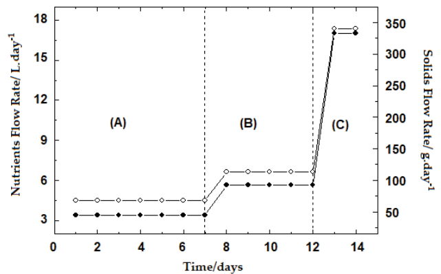
Figure 3 - Profile of the continuous production of Mesophilic Microorganisms, over a period of 14 days. The solid symbols (●) represent the Nutrient Feed and the empty symbols (○) the Solids, obtaining the following retention times (A) 5 days; (B) 3 days and (C) 1 day.
