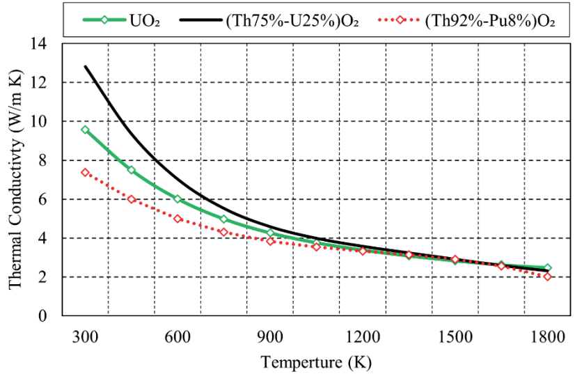
Figure 1: Thermal conductivity of UO 2 , (Th75%-U25%)O 2 and (Th92%-Pu8%)O 2 .
