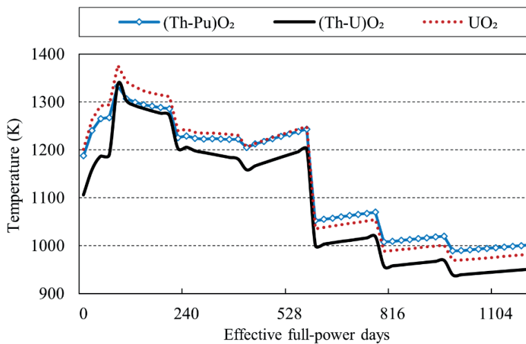
Figure 2: Comparison of fuel center temperature during the full burn cycle.
