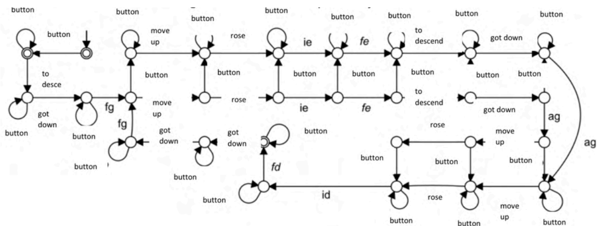
Figure 7: Monolithic supervisory control.
