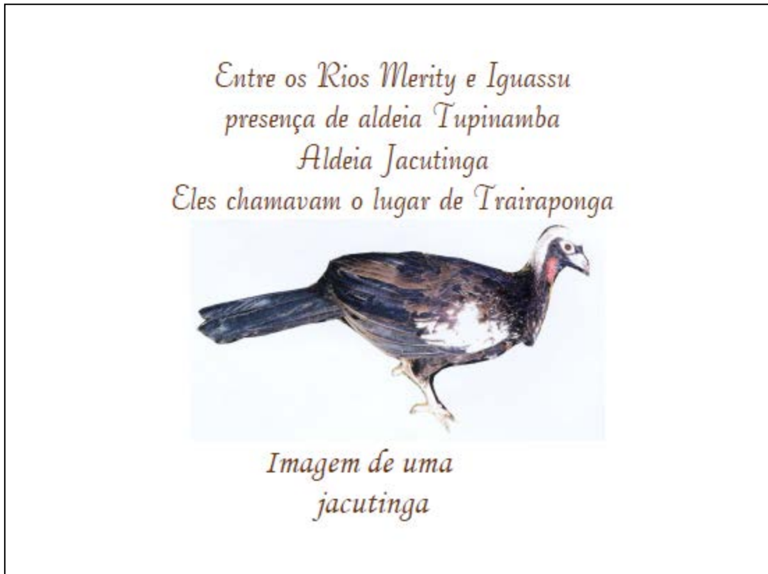
Figura 36 – Powerpoint
