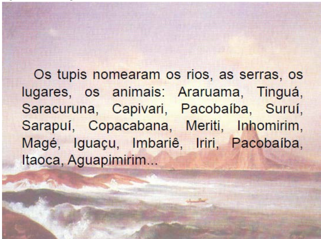
Figura 37 – Powerpoint
