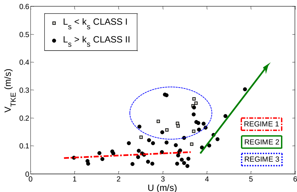
Figure 10. Scheme of the V_{TKE} \times U plot presenting the three turbulence regimes applied to the Uatumã site data (each regime is associated with a color indicated on the right down panel). The dashed line on the left represents the Regime 1, the continuous line on the right indicates the Regime 2 and the points inside the ellipse are associated with the Regime 3. The black dots represent the CLASS II GWs events and the grayscale rectangles represent the CLASS I ones.
