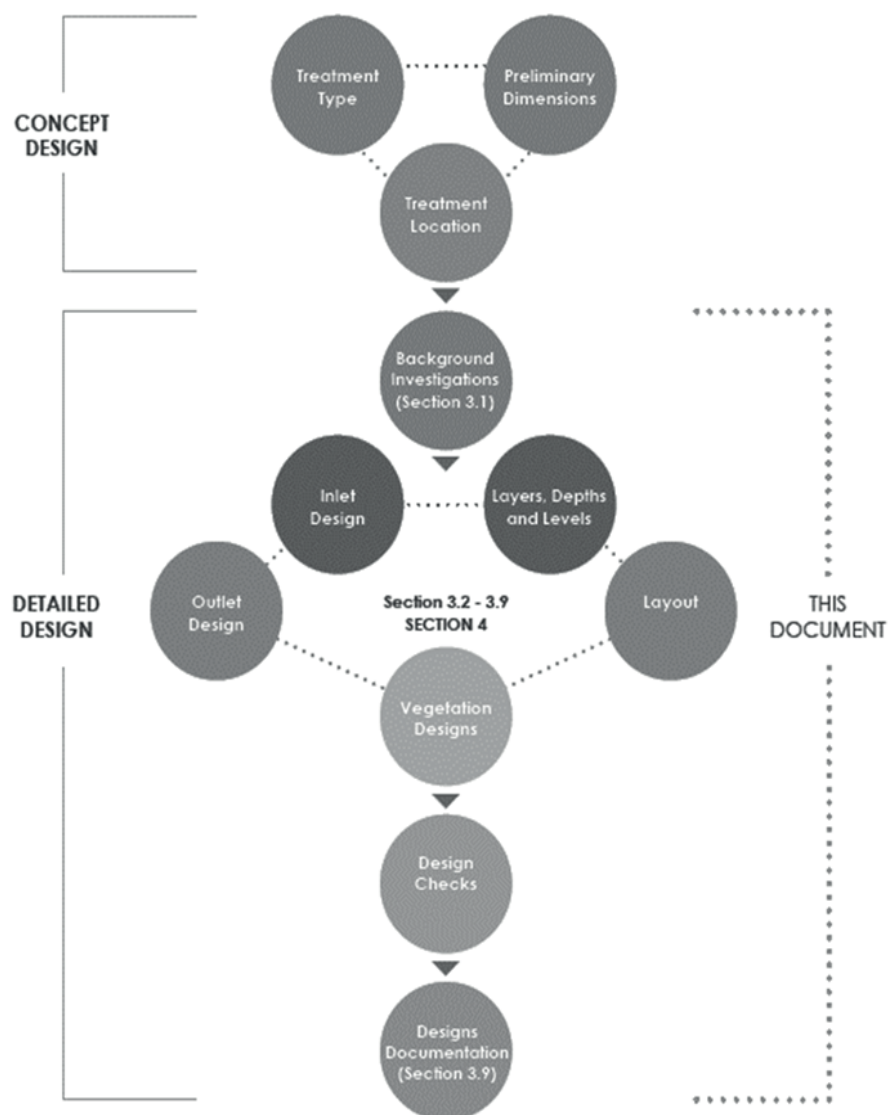
Fig.1: Wetland design process, pág. 23. (Wetland Technical Design Guidelines, 2017).
